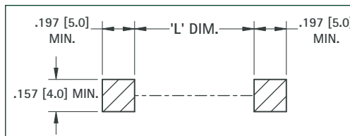
Pad Layout
