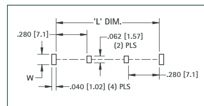
Mounting Detail
